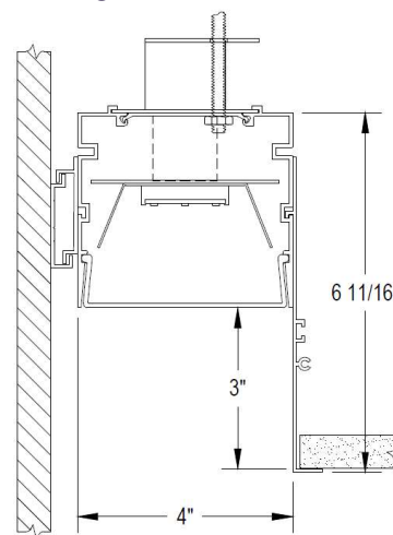
GPD4 4" Housing Width Regress 0", 1", 2", 3"
