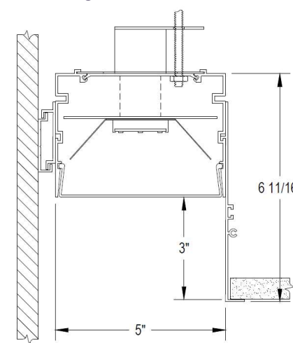
GPD5 5" Housing Width Regress 0", 1", 2", 3"
