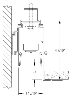
GPD1 1.8" Housing Width Regress 0", 1"
