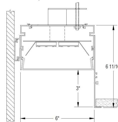
GPD6 6" Housing Width Regress 0", 1", 2", 3"
